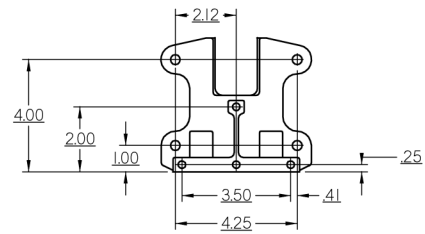
1 PEDAL, 2 MASTER CYLINDERS PEDAL ASSEMBLY P/N 72-604
