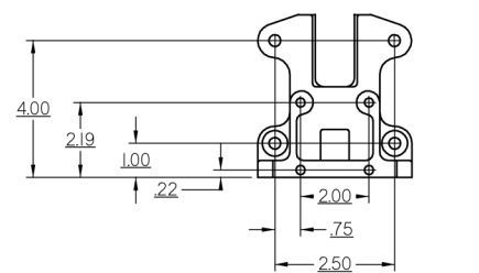
1 PEDAL, 1 MASTER CYLINDER PEDAL ASSEMBLY P/N 72-672
