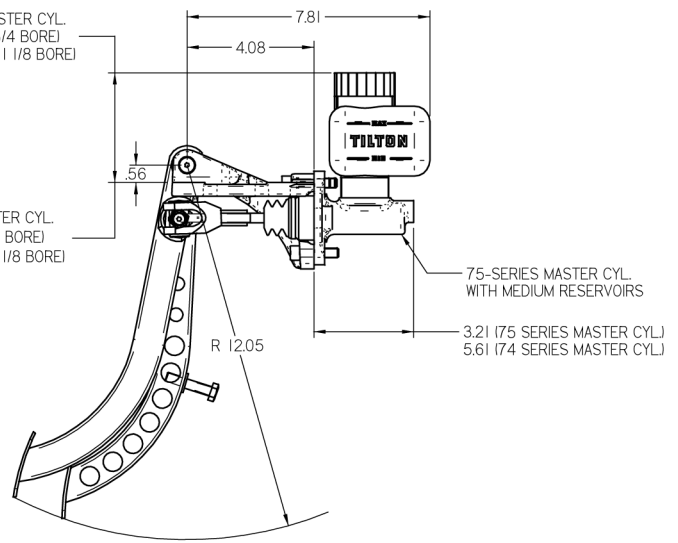
1 PEDAL, 1 MASTER CYLINDER PEDAL ASSEMBLY P/N 72-672
